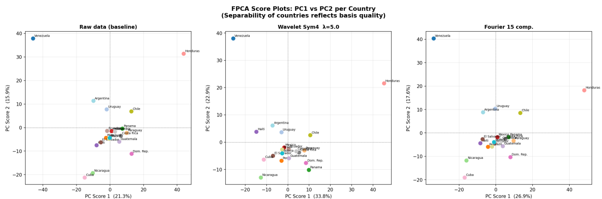
Figure 5.13: Score plots (replicating Fig 8 of paper).
