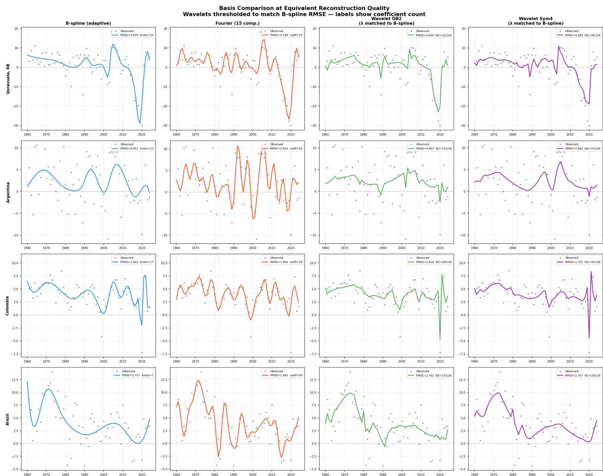
Figure 5.5: Basis comparison grid.
