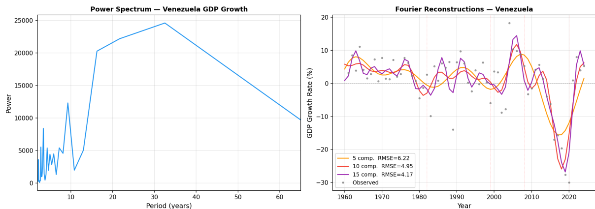
Figure 5.9: Fourier spectrum — Venezuela.
