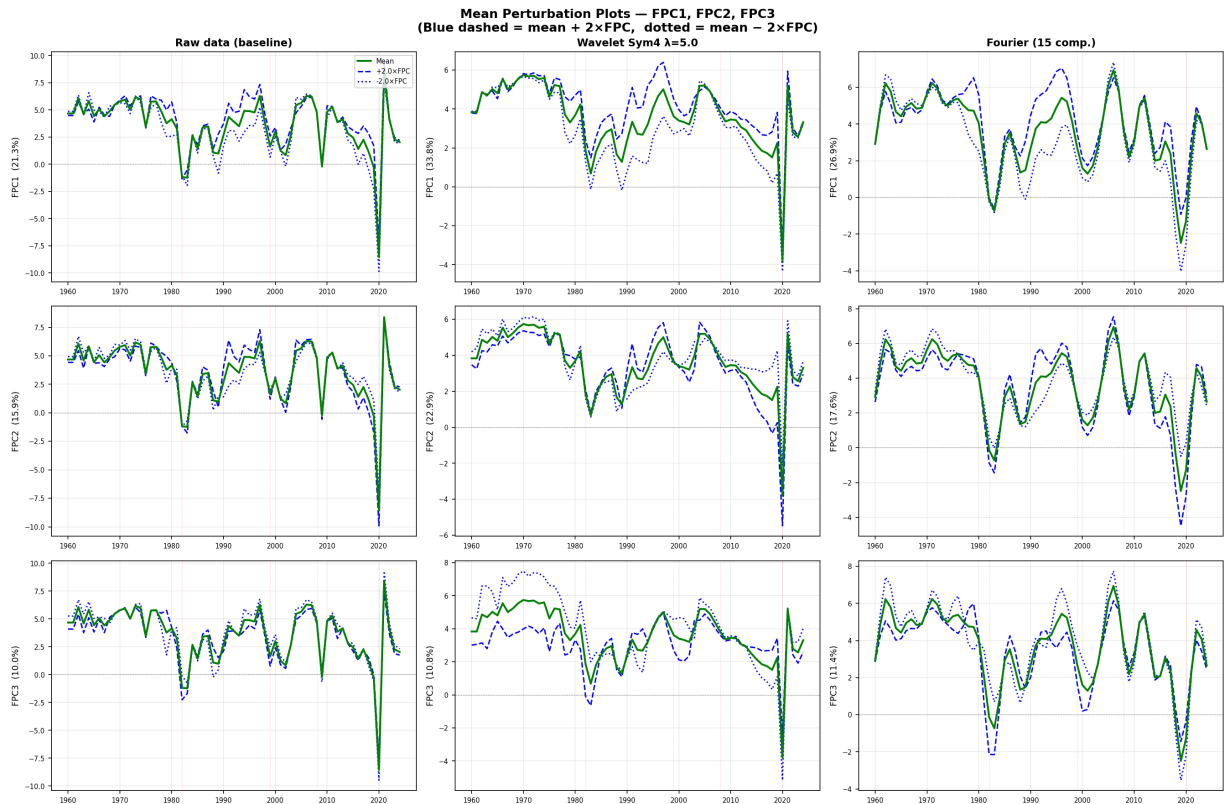
Figure 5.12: FPC curves (perturbation plots).
