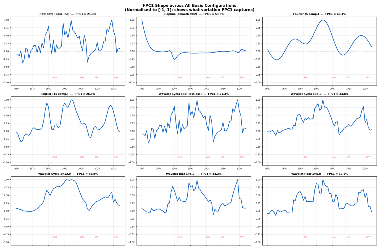
Figure 5.11: FPC1 curve comparison across bases.
