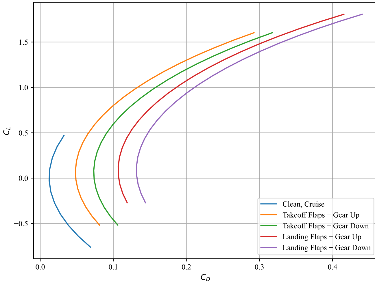
Drag Polar for F/A-24 Hyper-Hornet
