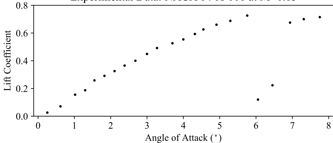
Experimental Data: NACA 64-A-006 at M=0.85
