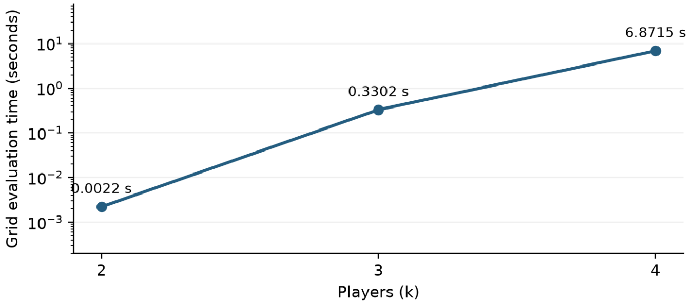
Figure 1. Measured payoff-tensor construction time for each original grid size, on the host specified in section 3.1.3. The times are 0.0022, 0.3302, 6.8715 seconds for k = 2, 3, 4 . They exclude the subsequent candidate-certificate stage. Every one of the 18,974,736 four-player angle profiles is evaluated. Batched NumPy operations and small statevectors make these CPU computations practical. The three grids have different resolutions, and these isolated runs do not establish an asymptotic scaling law or a controlled speedup over historical implementations.
