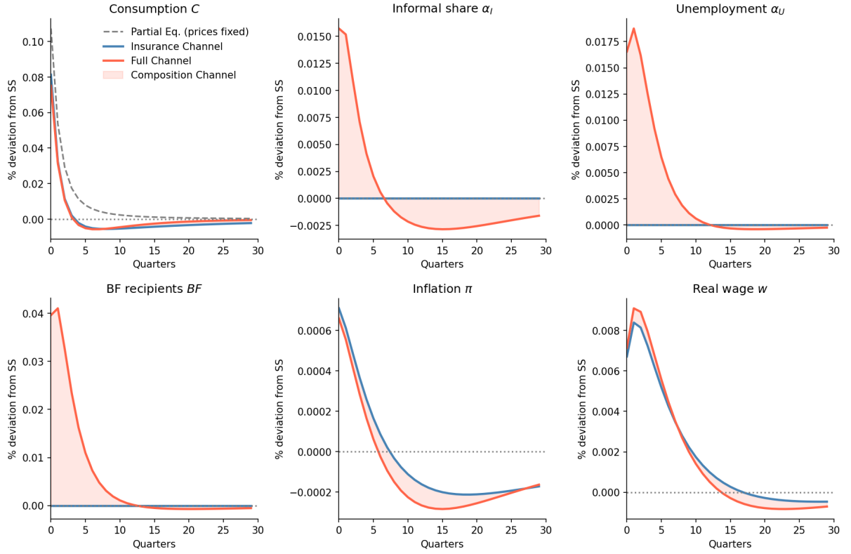
Figure 5: IRFs: Insurance vs Composition Effect (shock in T )
