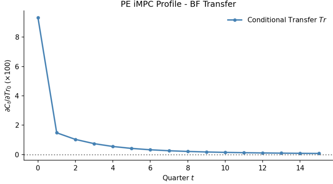
Figure 4: Partial Equilibrium iMPC
