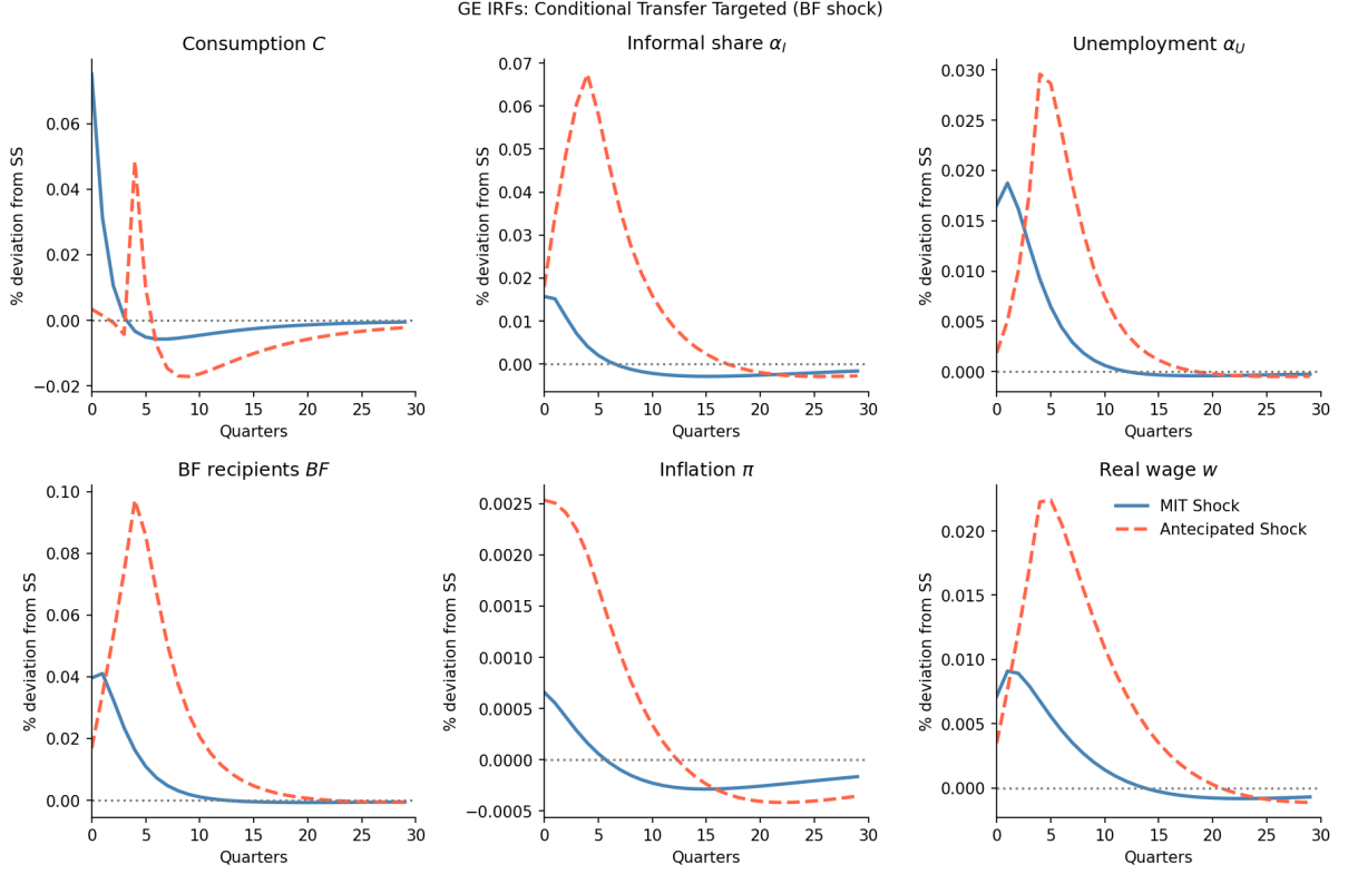
Figure 6: IRFs: MIT vs Anticipated Shock (shock in T )
