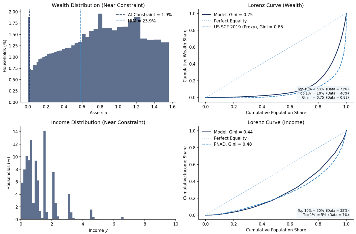
Figure 10: Wealth Distribution
