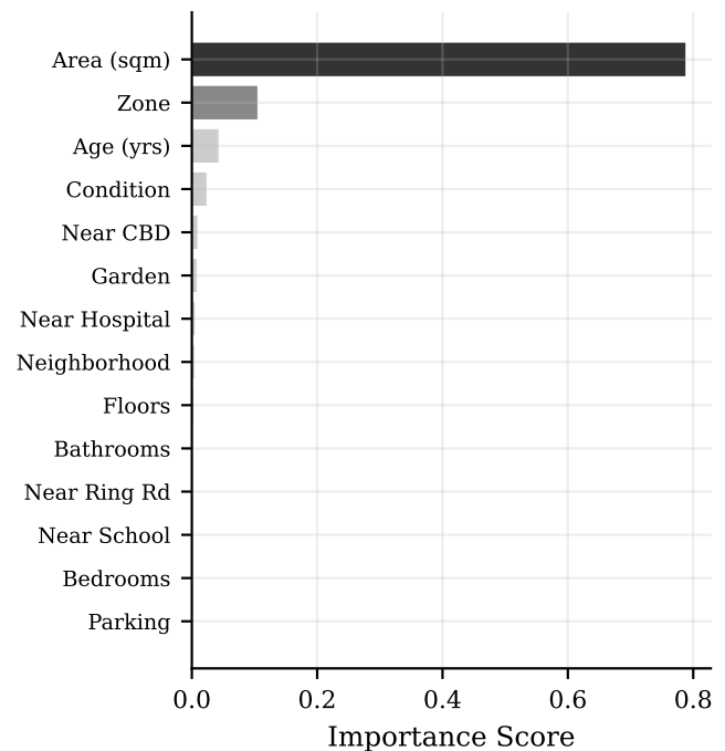
Fig. 6. Feature importance scores from Gradient Boosting. Darker bars indicate higher contribution to prediction accuracy.
