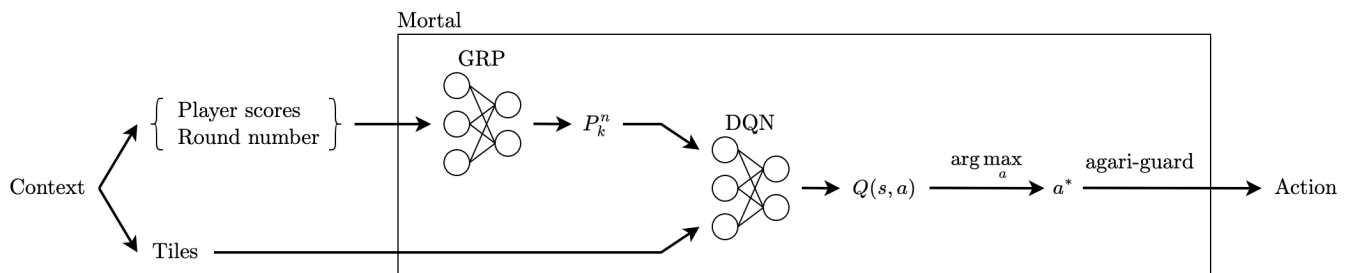
図 4: A diagram of how Mortal AI makes its decision.
