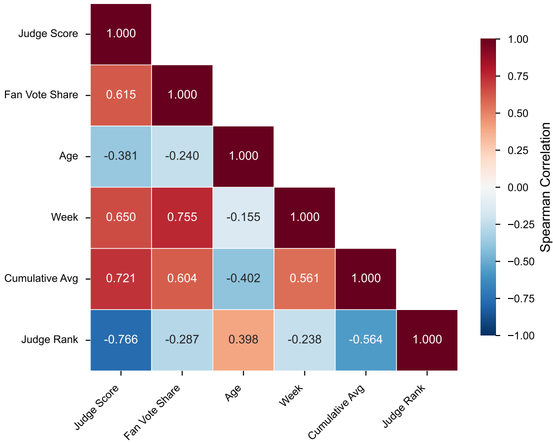
Feature Correlation Heatmap (Spearman)
