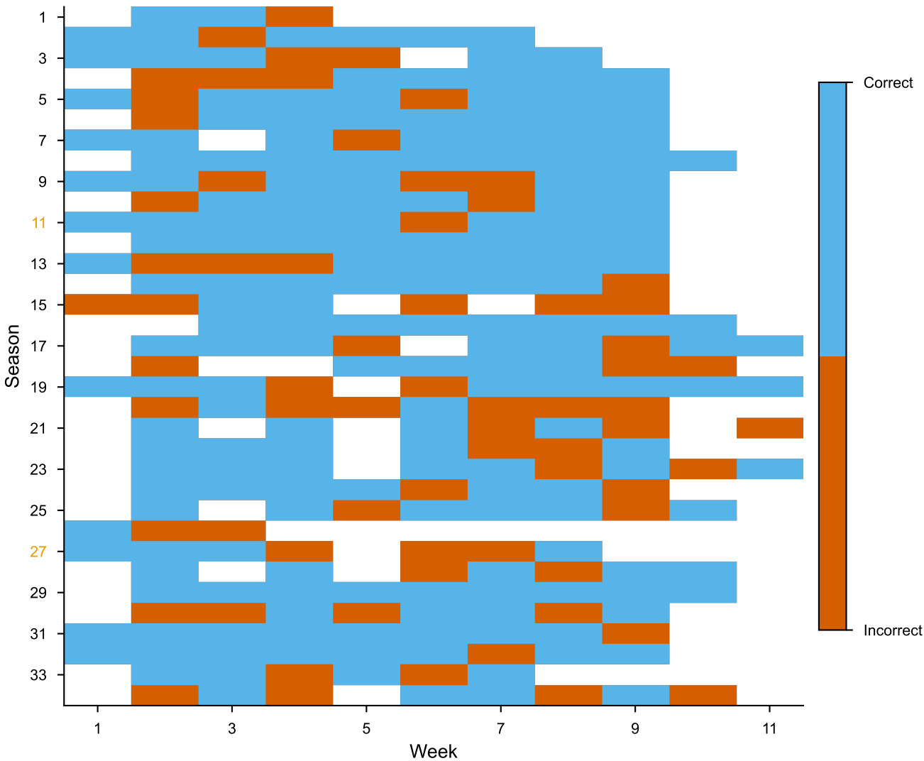
Consistency heatmap (Rank Sum vs actual elimination)
