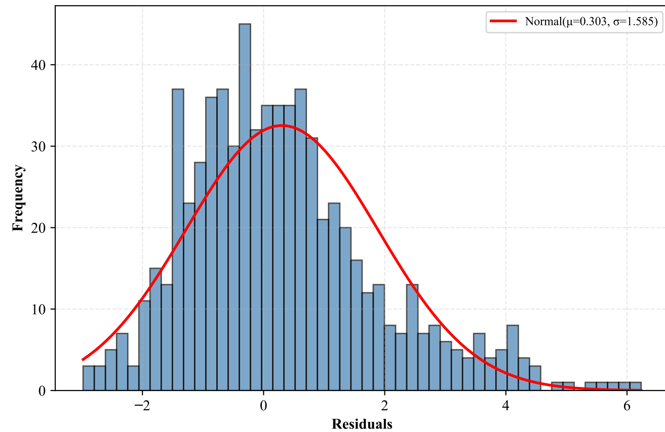
SVR - Residual Distribution
