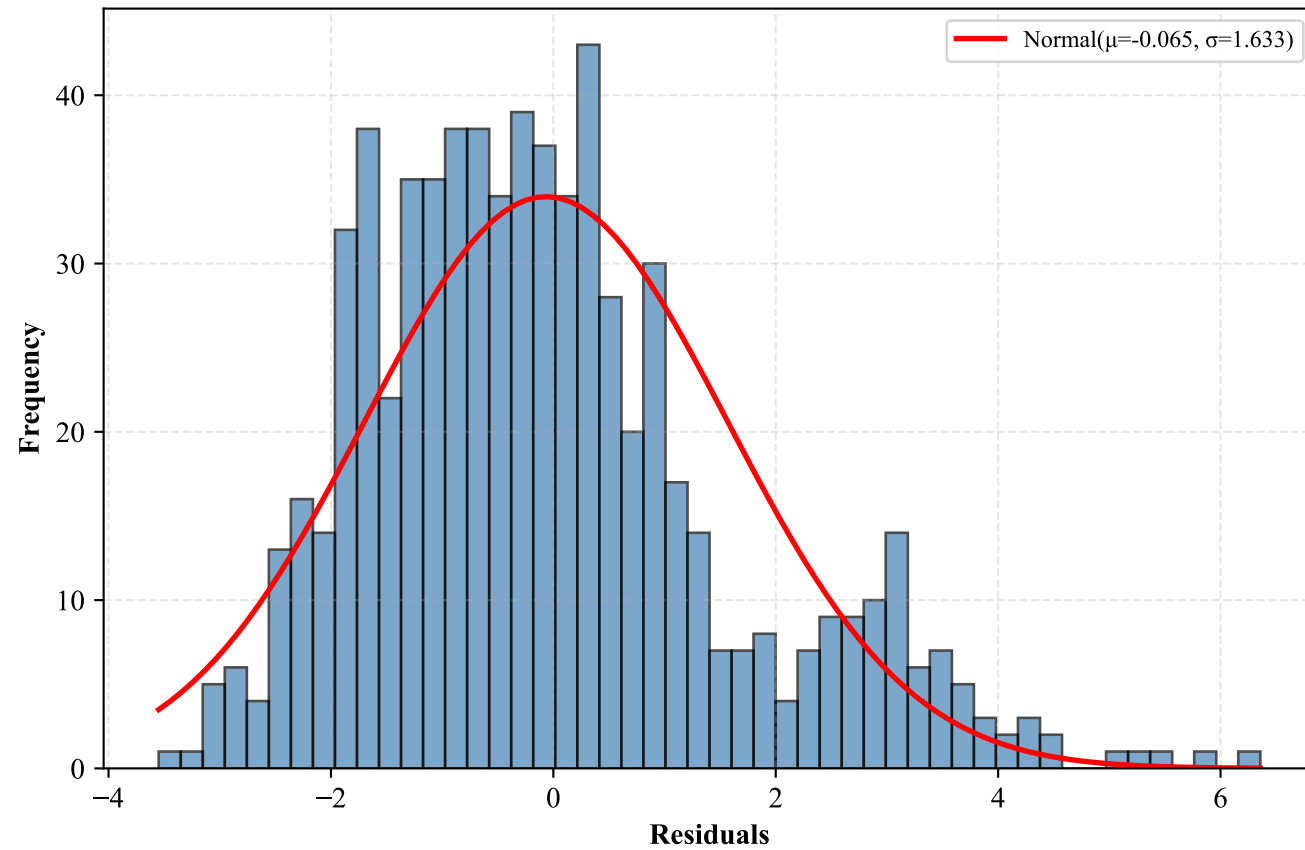
ElasticNet - Residual Distribution
