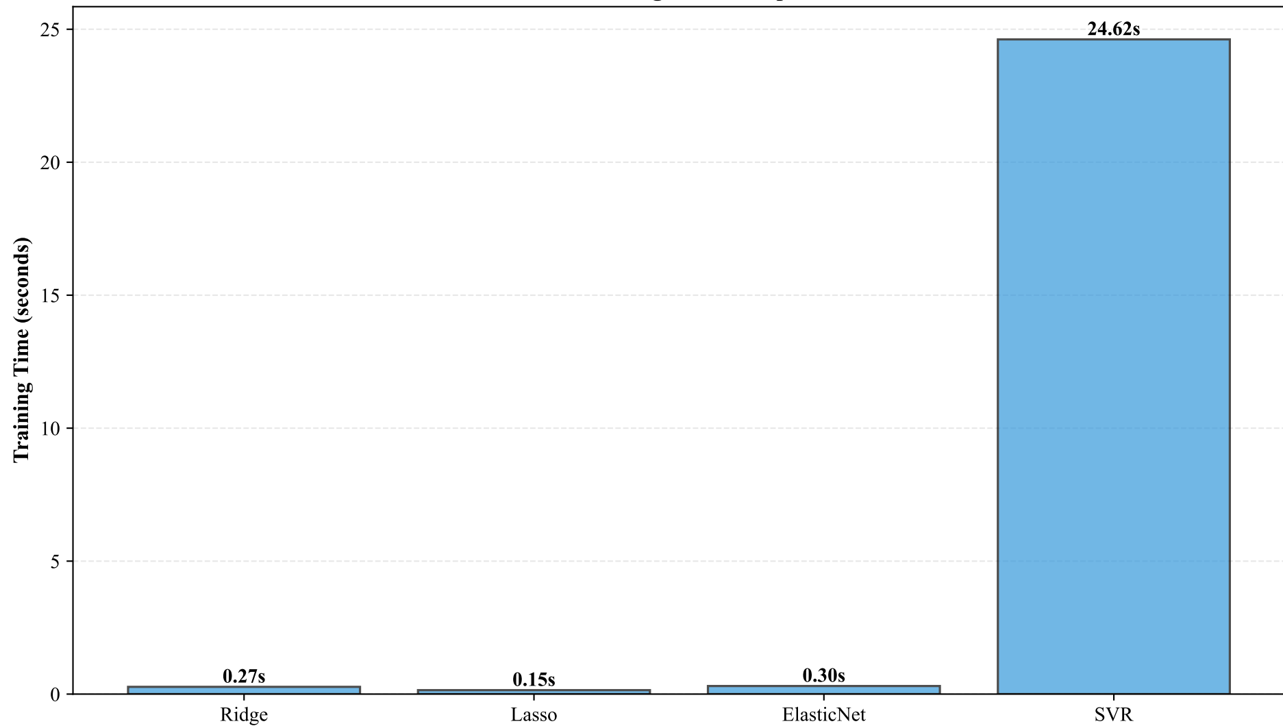
Model Training Time Comparison
