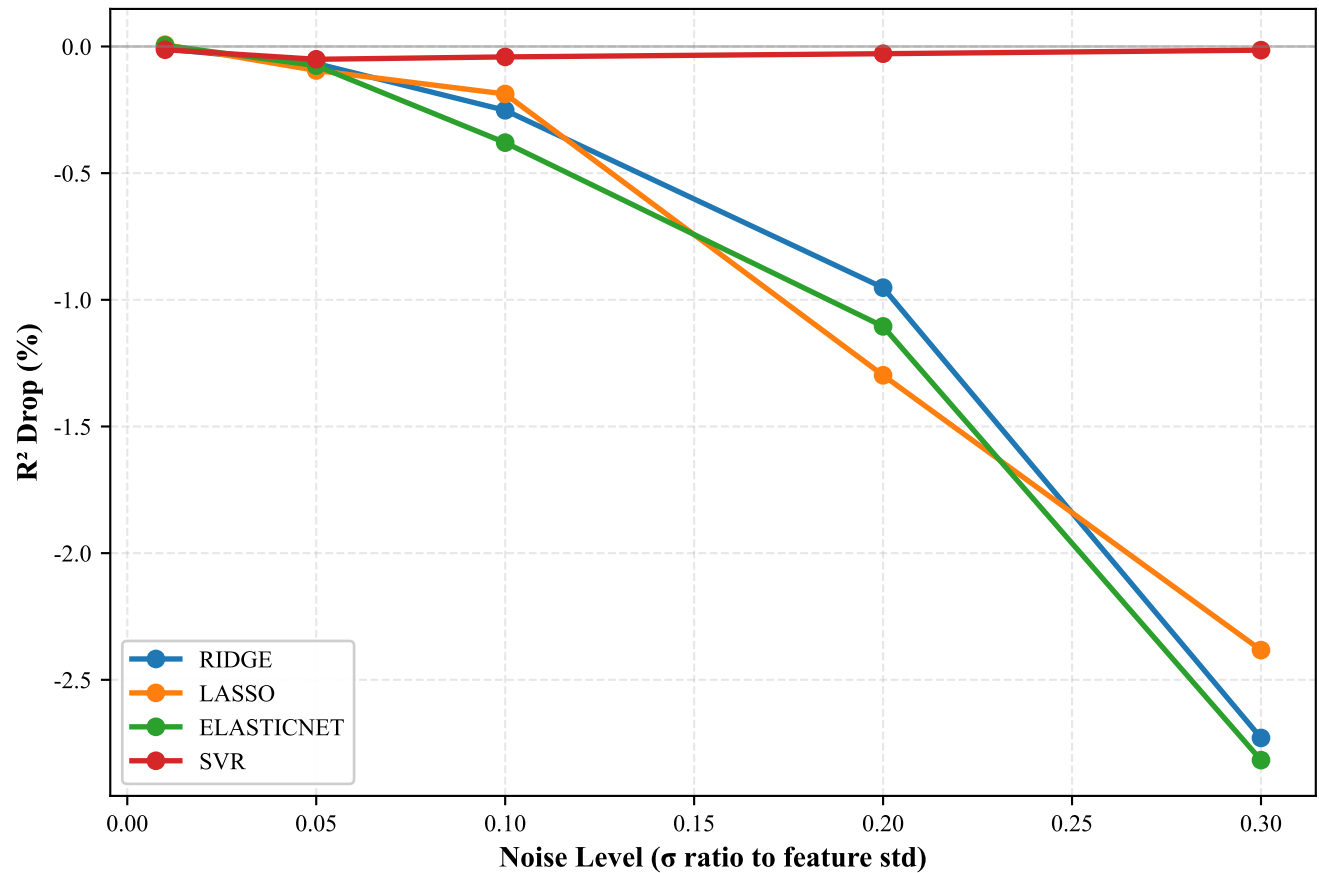
(B) Performance Degradation
