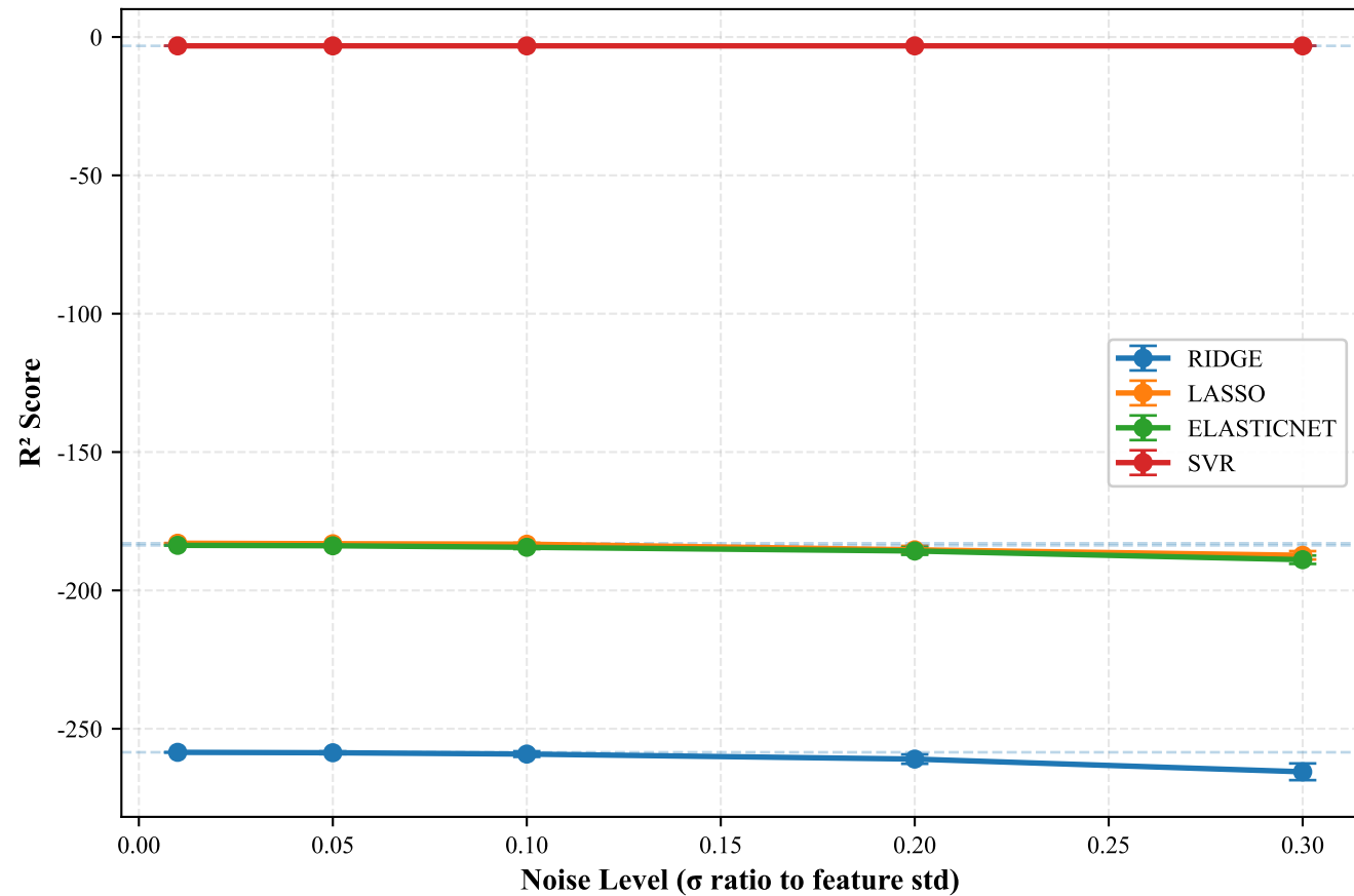
(A) Model Performance under Gaussian Noise
