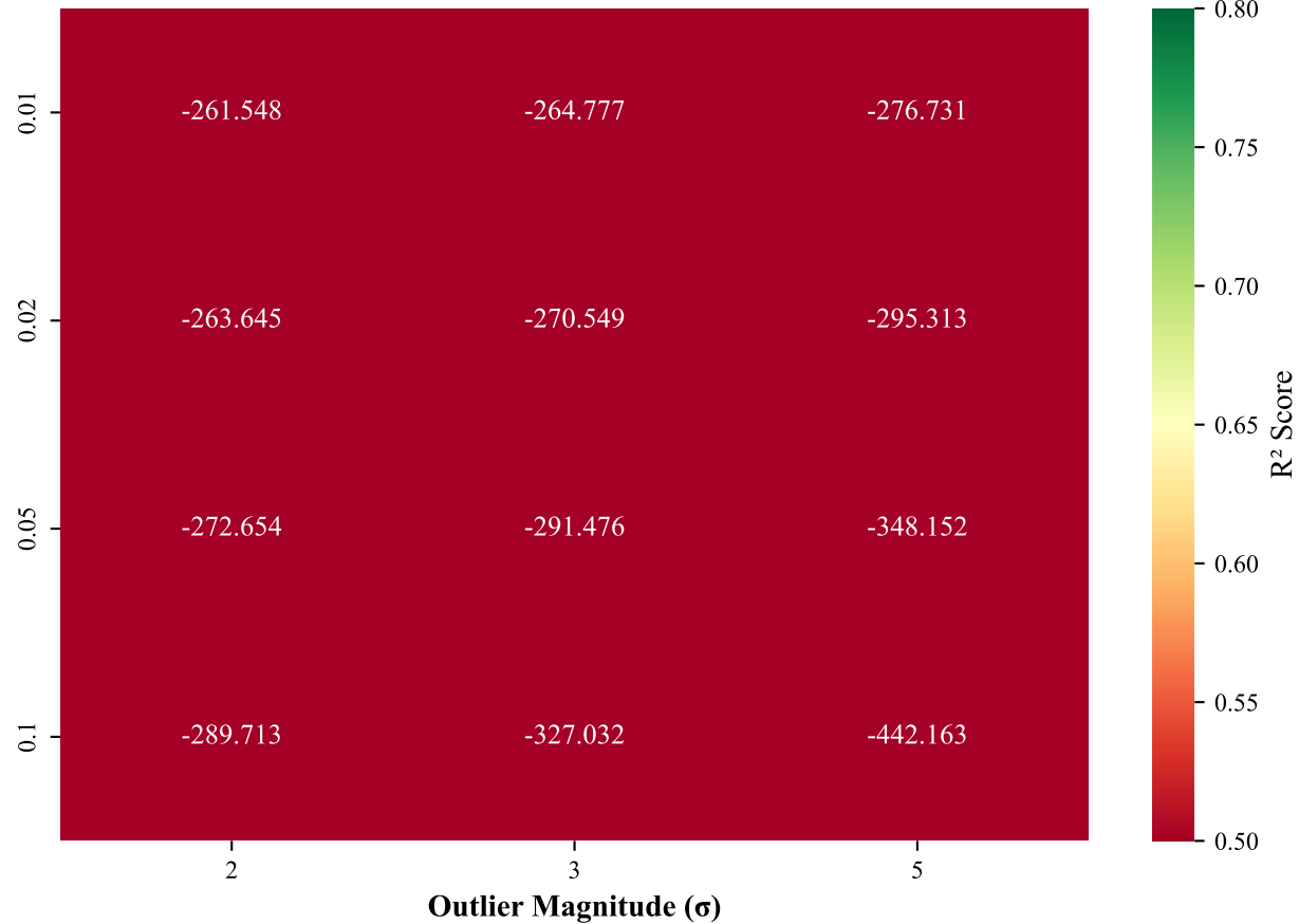
(A) RIDGE: Outlier Rate \times Magnitude
