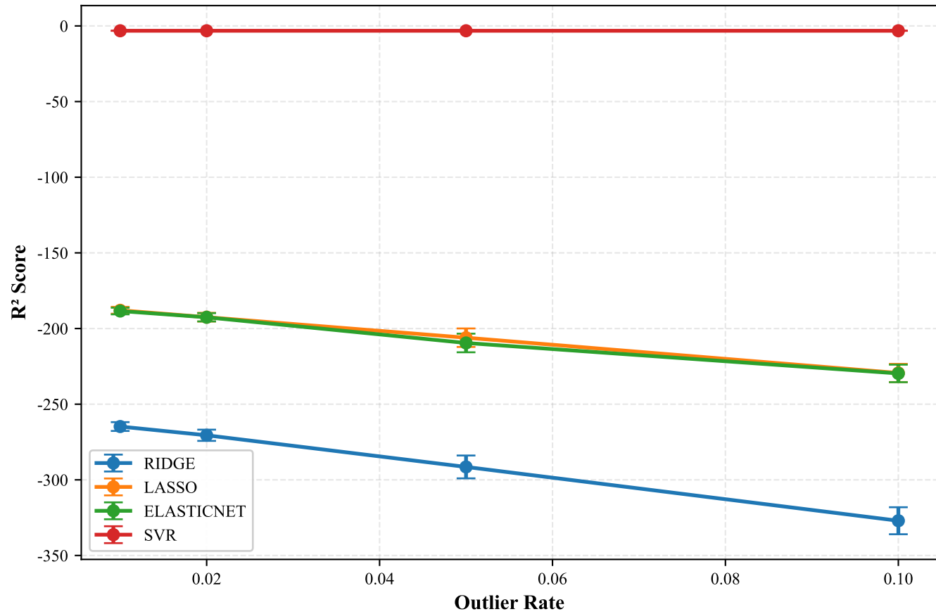
(B) All Models: Performance vs Outlier Rate ( 3\sigma )
