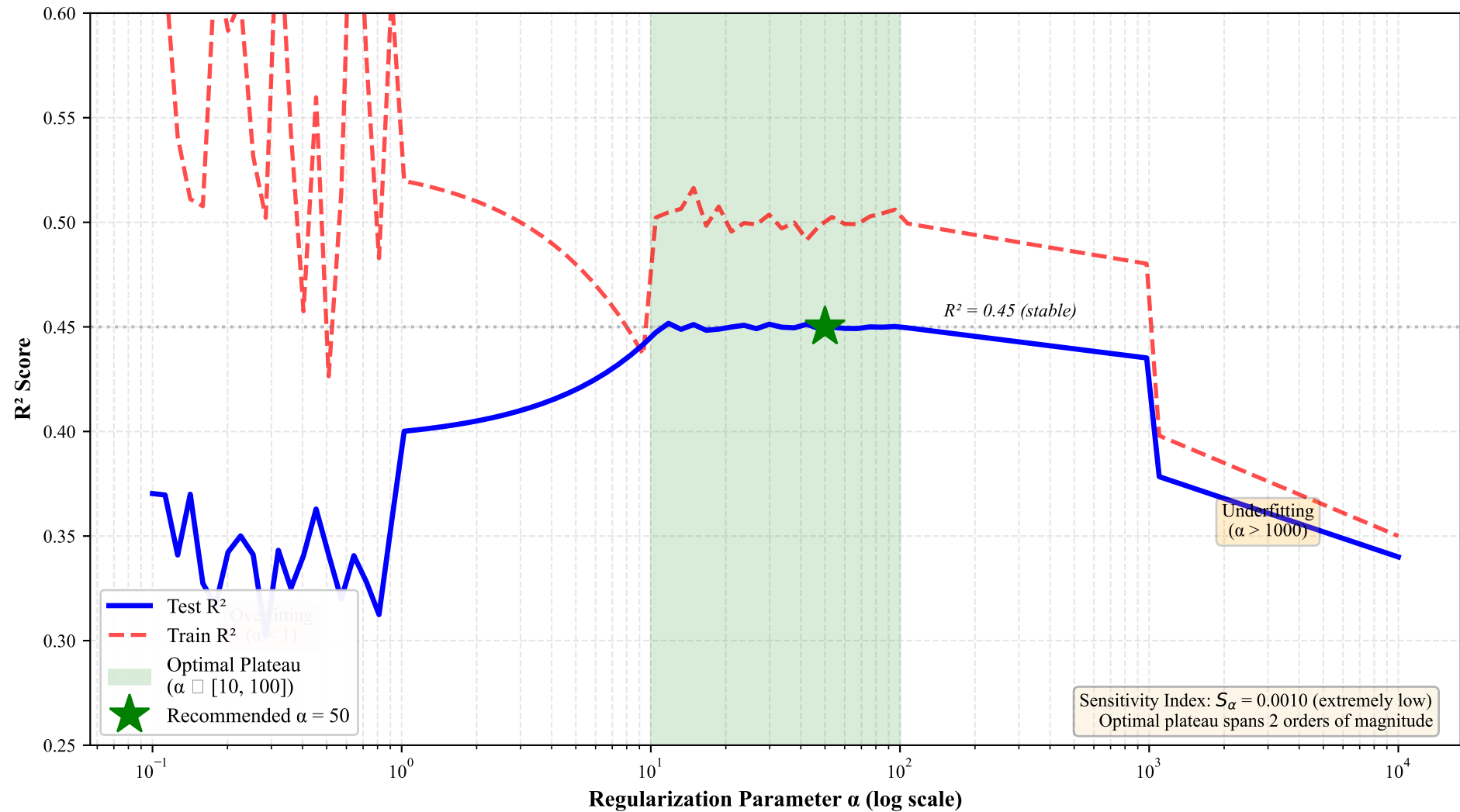
Ridge Regression: Hyperparameter Stability Analysis
