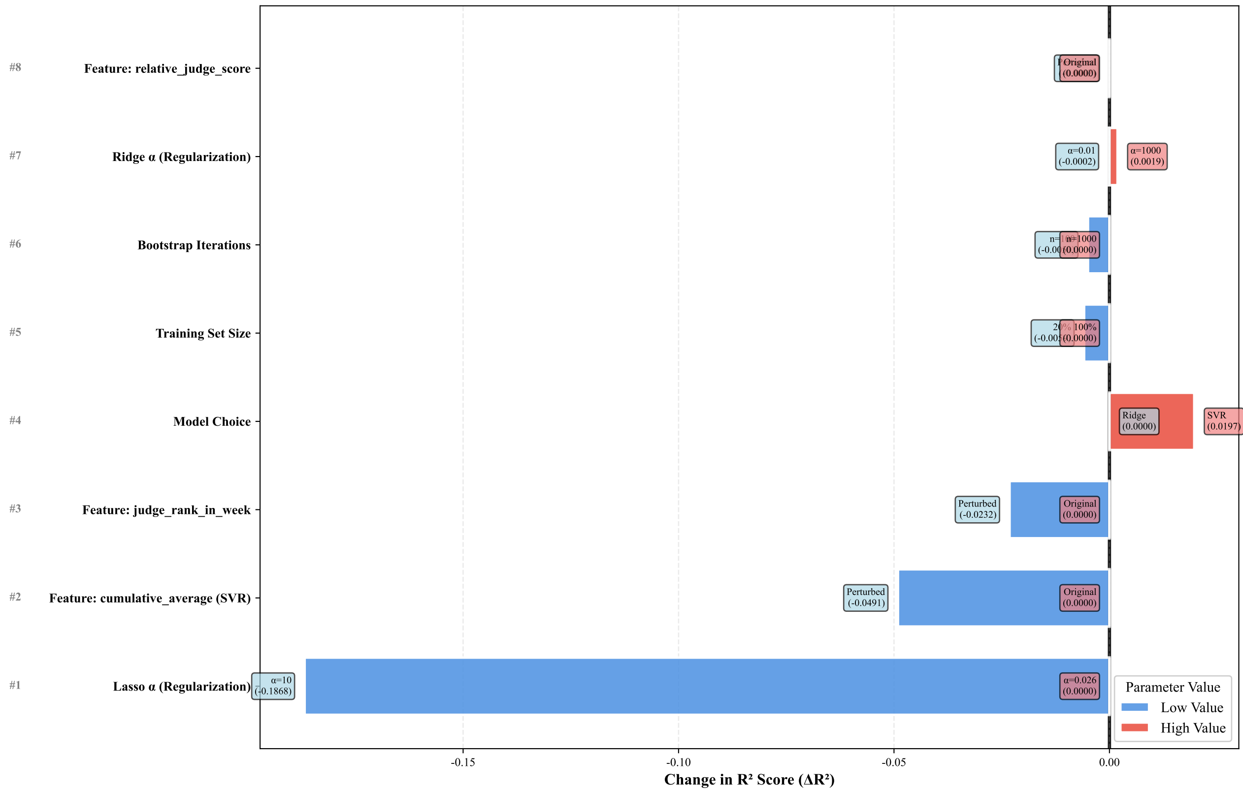
Parameter Sensitivity Analysis: Impact on Model Performance
