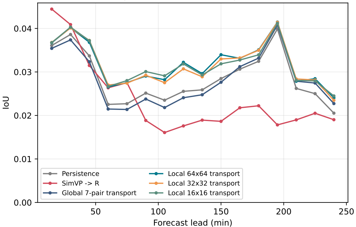
Thick-cloud pixel IoU (CPP \geq 30 , prediction \geq 30 )
