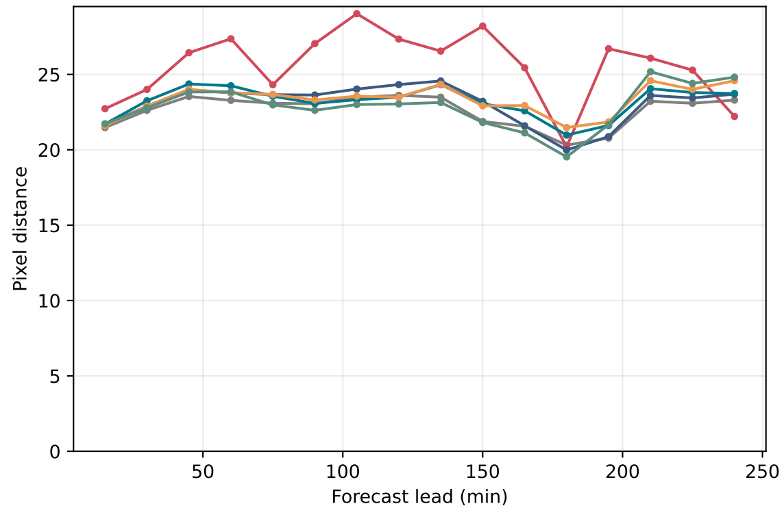
Cloud-mask centroid distance
