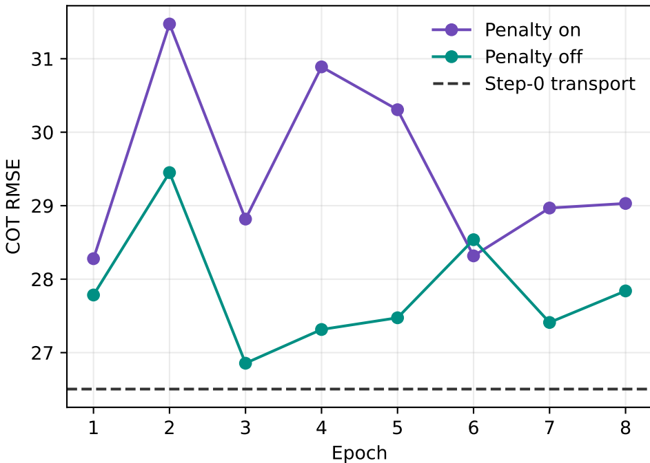
Thick-cloud RMSE (CPP COT \geq 30 )
