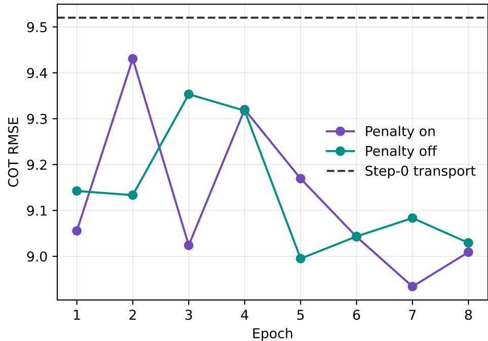
All-valid COT RMSE
