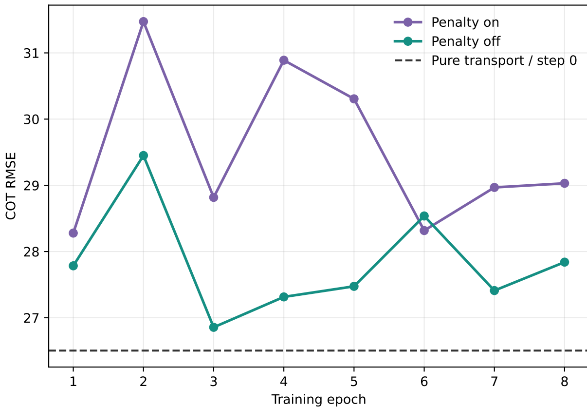
Thick-reference COT RMSE (COT \geq 30 )
