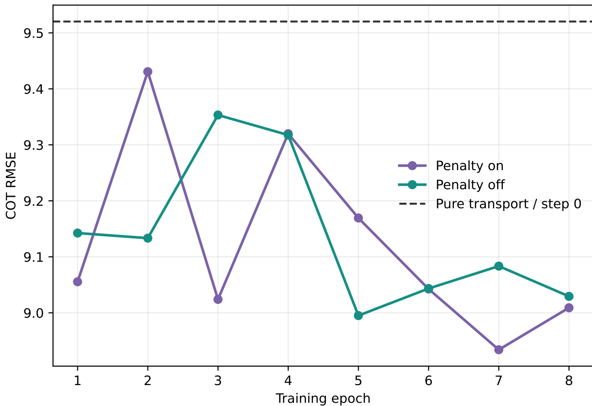
All-valid COT RMSE
