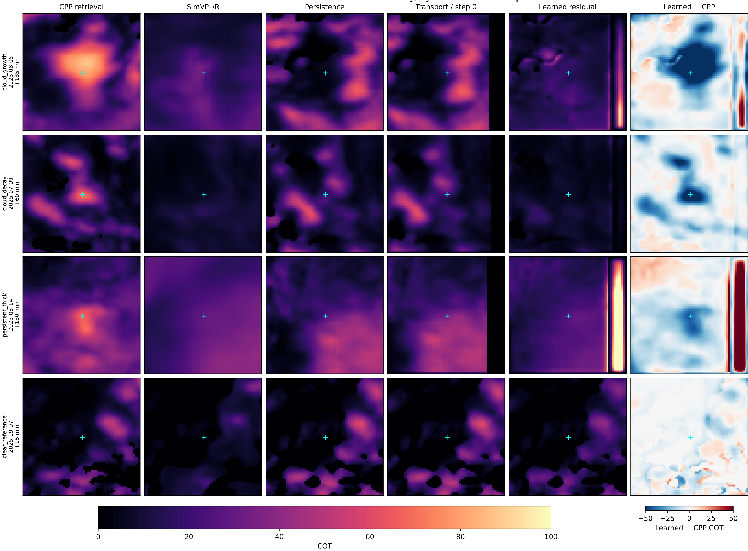
Sili local 64×64 COT cases — validation only; cyan cross = station pixel
