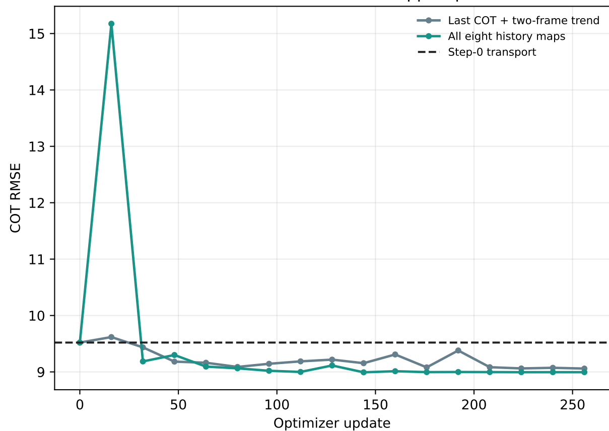
Patch RMSE on all common-support pixels
