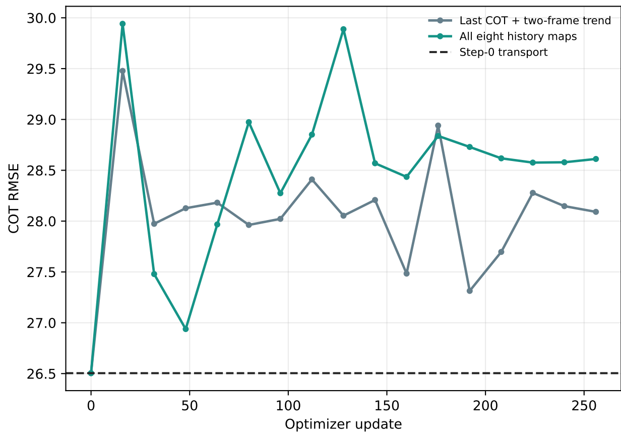
Patch RMSE on CPP COT \geq 30
