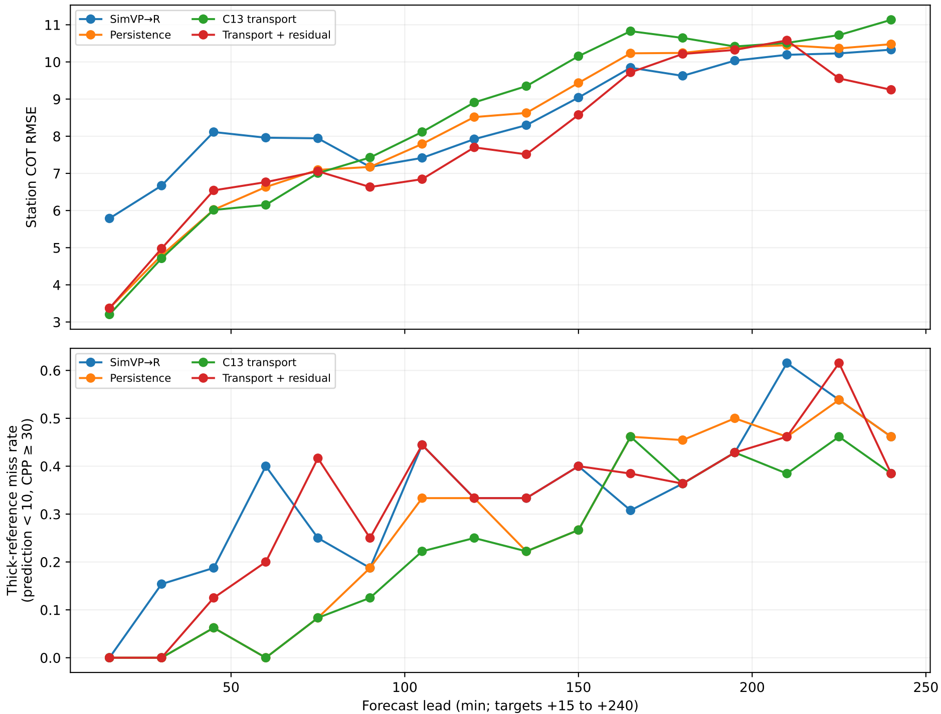
Sili station-pixel skill by lead — validation only
