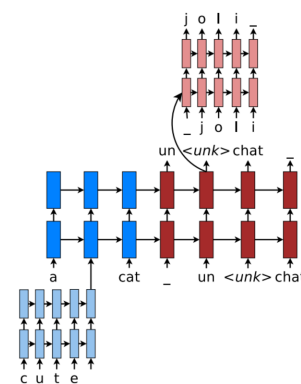
Figure 11: Hybrid NMT
