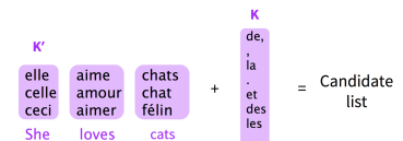
Figure 8: Candidate list
