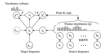
Figure 9: Pointer network Architecture
