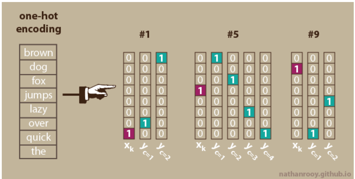
Figure 3: one-hot encoding
