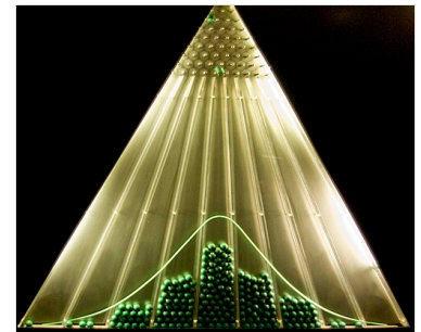
The bean machine , a device invented by Francis Galton , can be called the first generator of normal random variables. This machine consists of a vertical board with interleaved rows of pins. Small balls are dropped from the top and then bounce randomly left or right as they hit the pins. The balls are collected into bins at the bottom and settle down into a pattern resembling the Gaussian curve.
