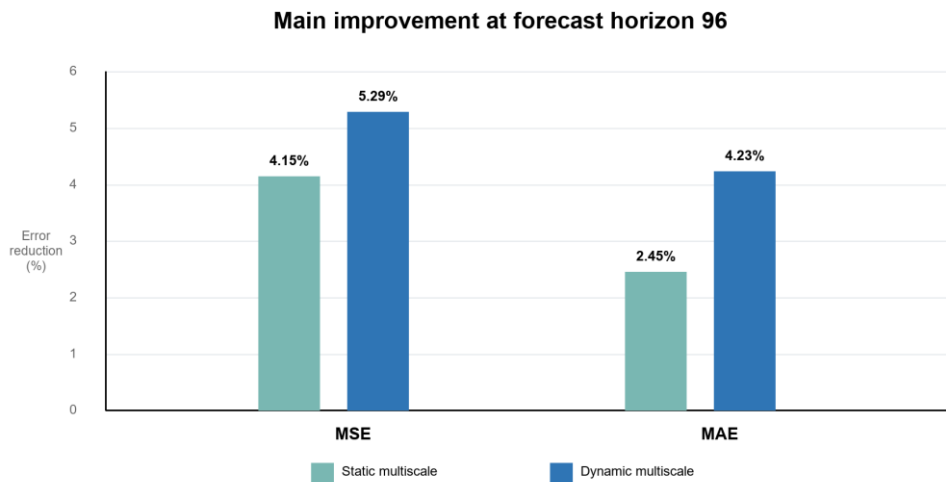
Figure 3. Mean paired error reduction at the main 96-step forecast horizon.
