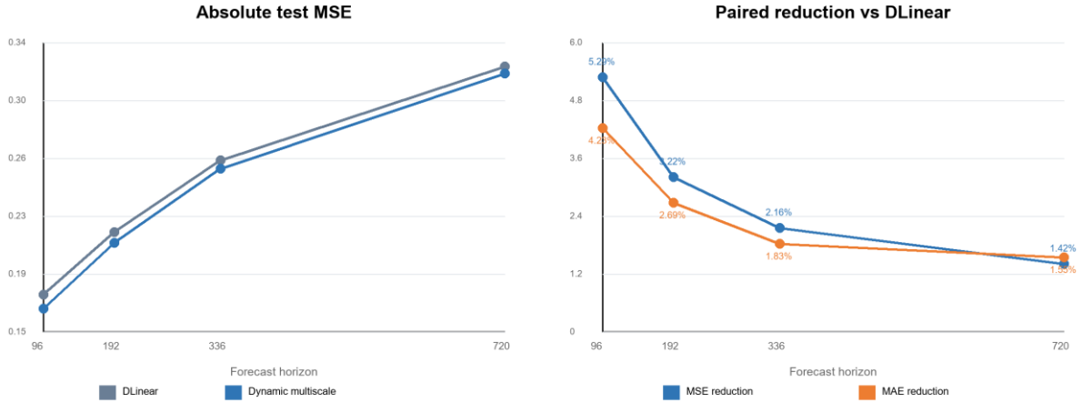
Figure 4. Absolute MSE and paired relative reductions across all evaluated horizons.
