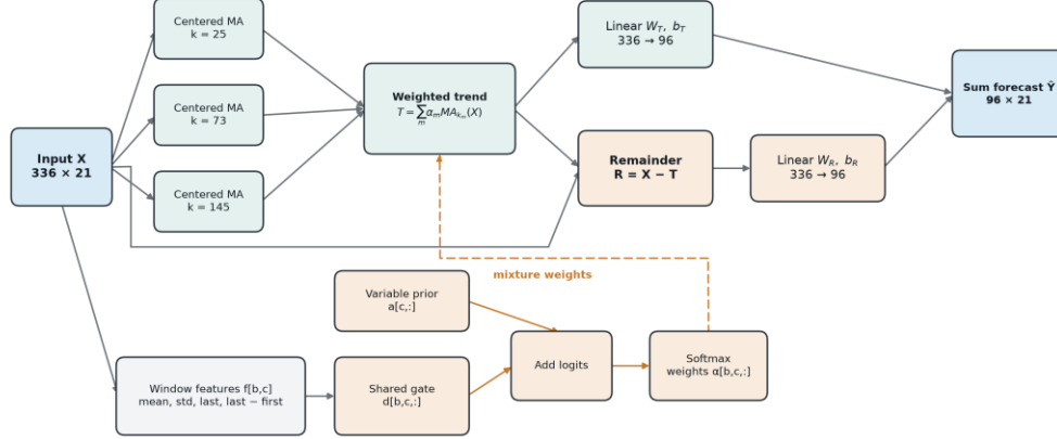
Figure 2. Proposed dynamic per-variable multiscale decomposition while retaining DLinear's forecasting layers.
