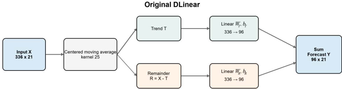
Figure 1. Original DLinear decomposition and direct multi-step forecasting flow.
