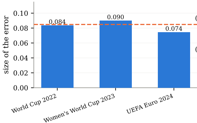
(a) The error travels between competitions
