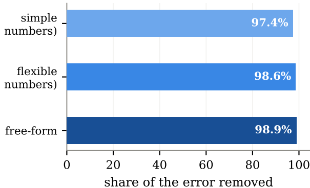
(b) ...and one correction fixes it
