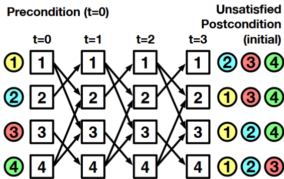
(c) Evaluate initial collective precondition and unsatisfied postcondition
