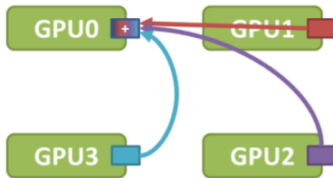
Reduce
