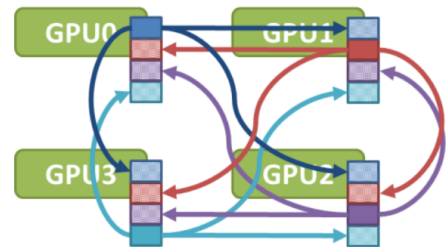
All-Gather
