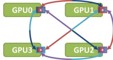
All-Reduce
