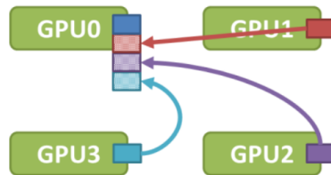
Gather
