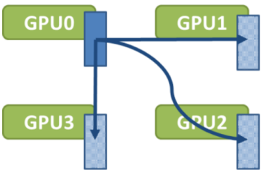
Broadcast
