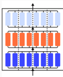
Expert Parallelism
