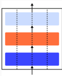
Tensor Parallelism
