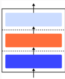
Pipeline Parallelism
