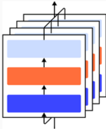
Data Parallelism
