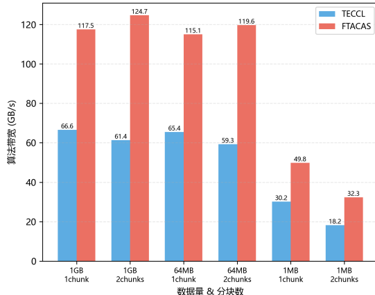
NDv2-4
