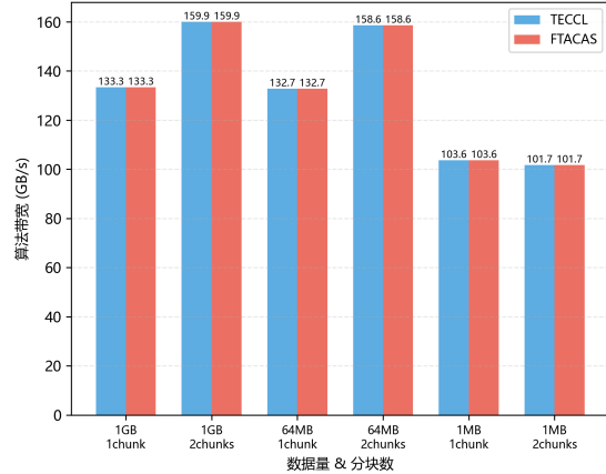
NDV2-2
