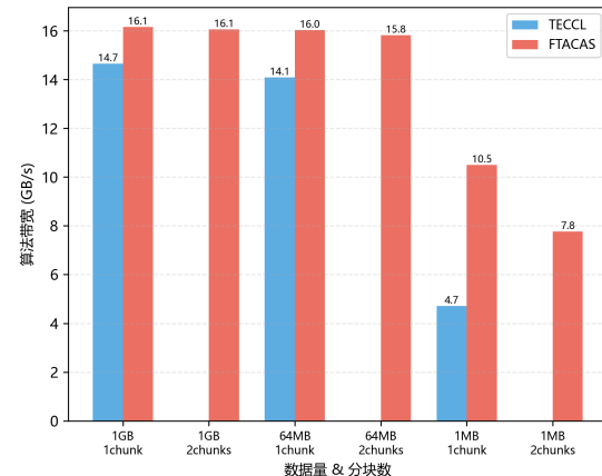
NDv2-4
