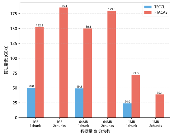
AMD-2
