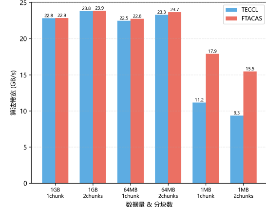
AMD-2
