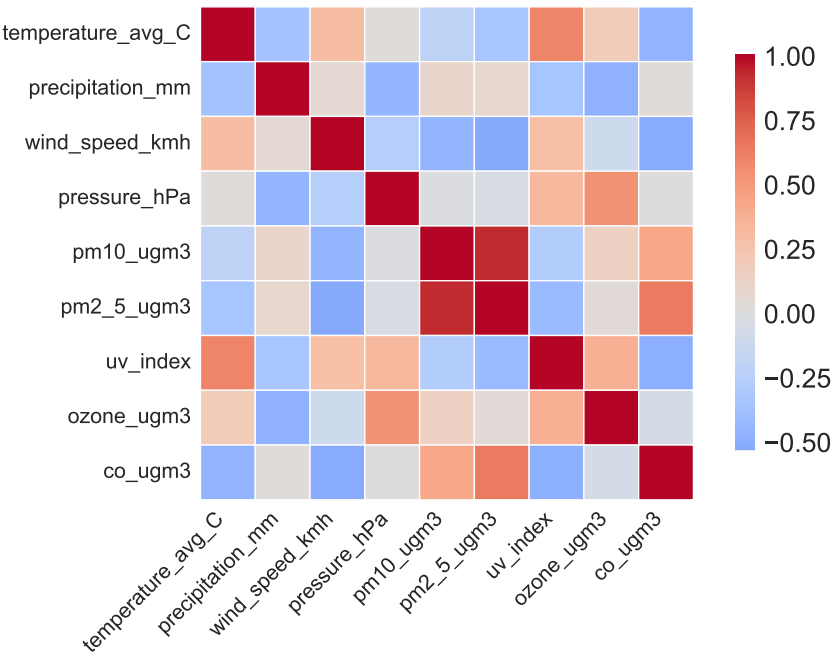
Correlation Matrix
