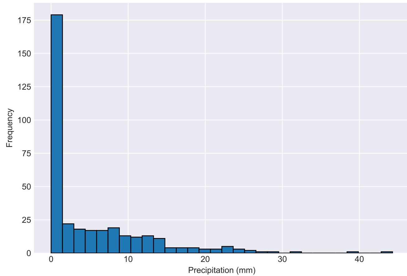
Precipitation Distribution
