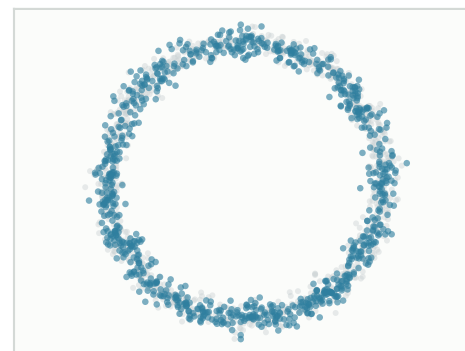
GMM
