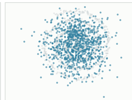
VAE
