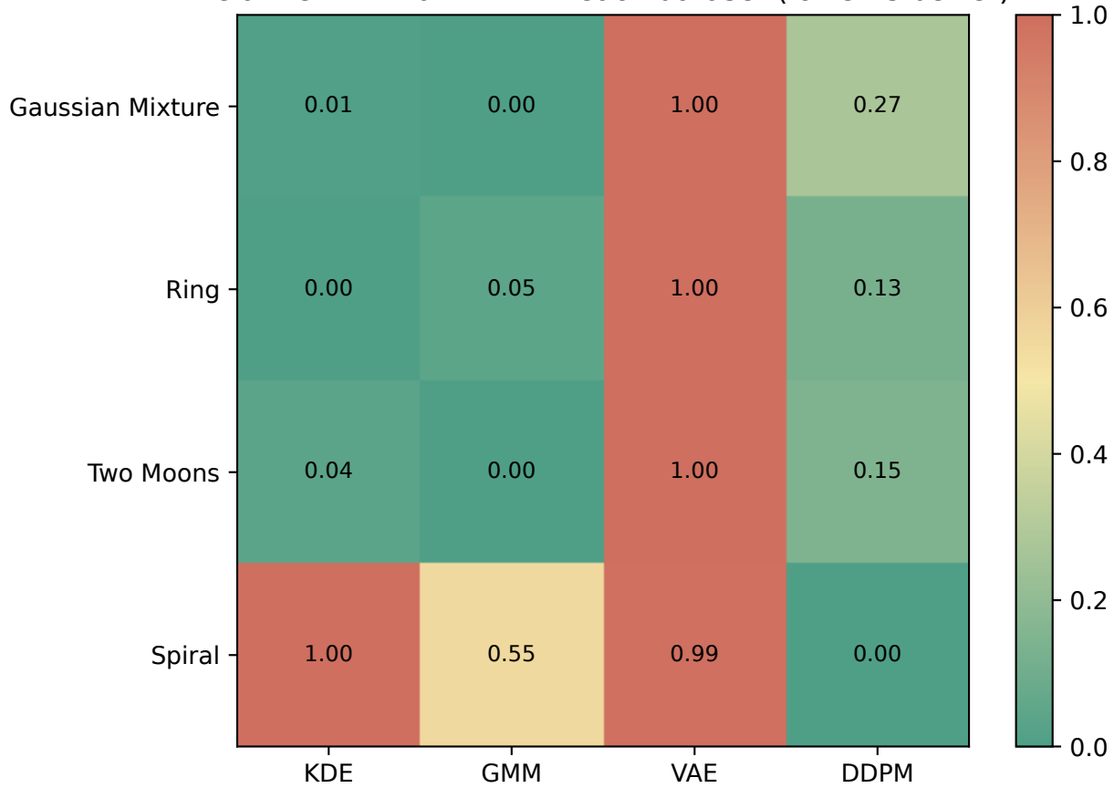
Relative MMD rank within each dataset (lower is better)
