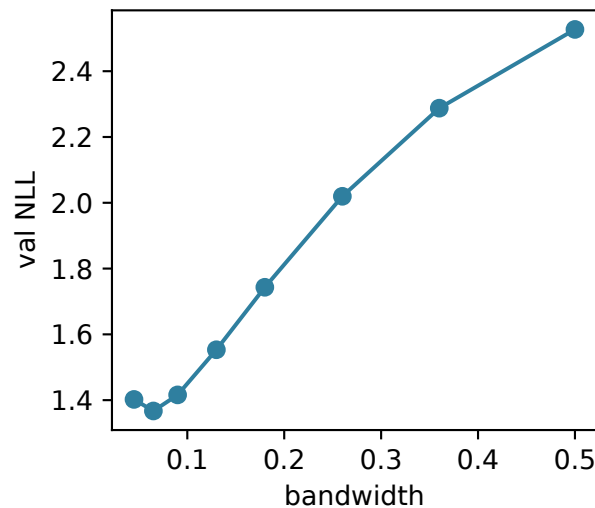
Two Moons GMM
