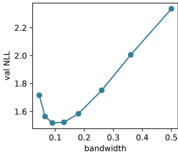
Gaussian Mixture GMM
