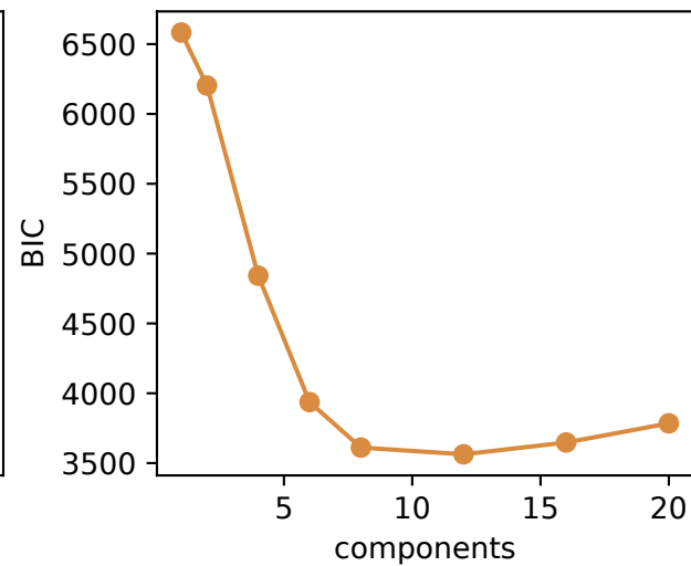
Two Moons GMM
