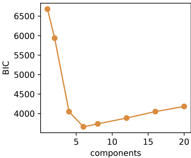
Gaussian Mixture GMM
