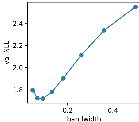
Two Moons GMM
