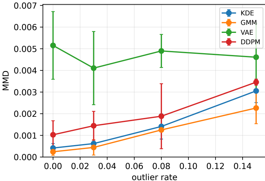
Two Moons
