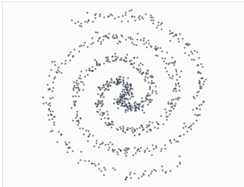
Spiral
