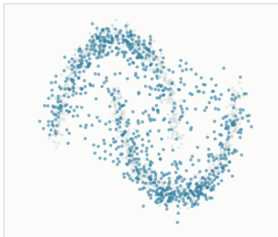
Conditional DDPM
