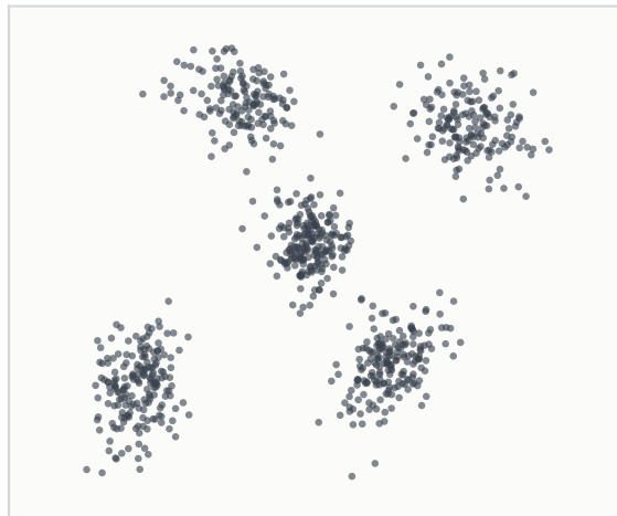
Conditional DDPM
