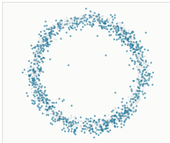
Conditional DDPM
