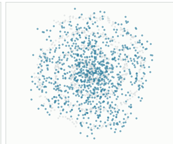
Conditional DDPM
