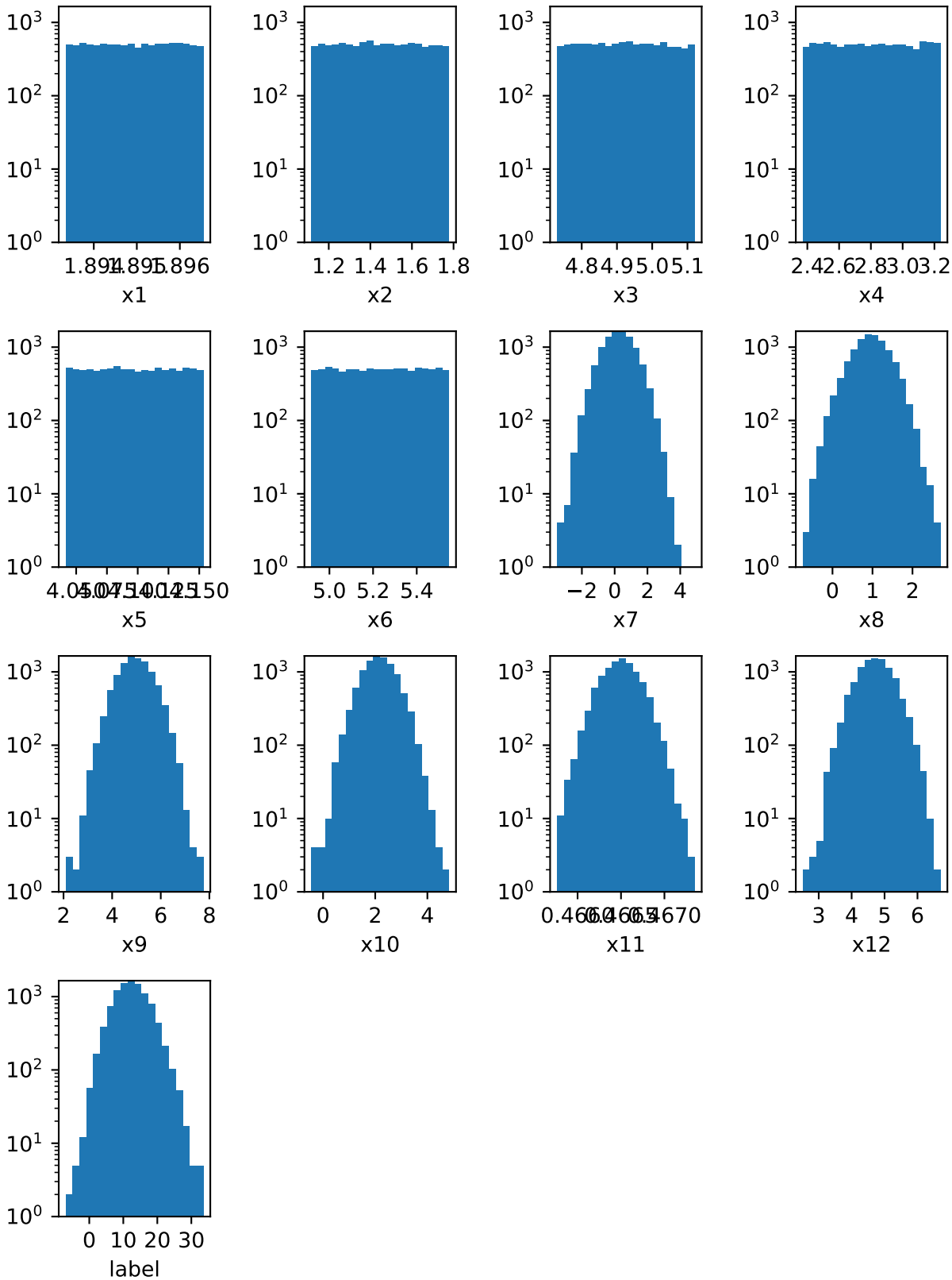
Feature Histograms
