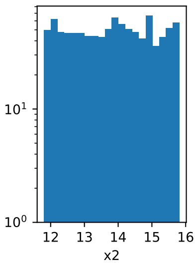
Feature Histograms
