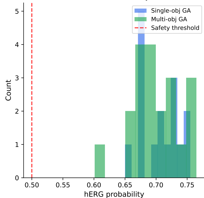
hERG Distribution Comparison
