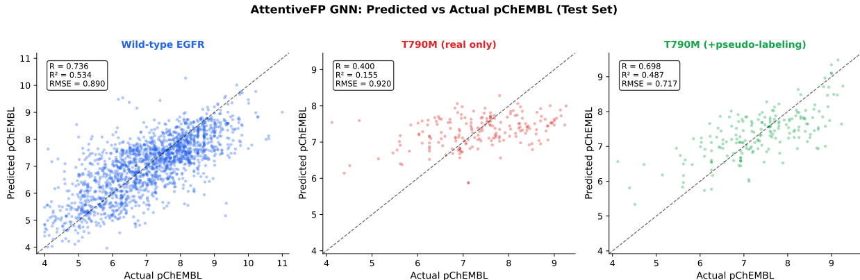
Figure 2: Predicted vs. actual pChEMBL values on the test set for three models. Left: wild-type EGFR ( R=0.736 , n=1,763 ). Center: T790M real-only ( R=0.400 , n=195 ). Right: T790M with pseudo-labeling ( R=0.698 , n=195 ). The sharp Pearson R recovery from pseudo-labeling is evident.
