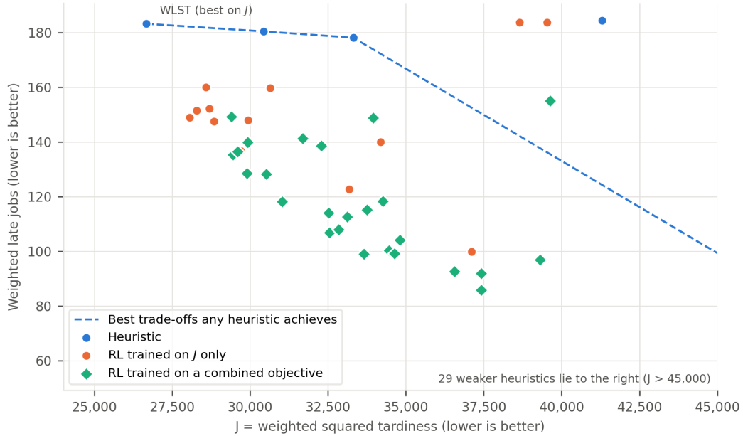
Figure 4: Offline, weighted jobs: J against the weighted number of late jobs (both lower is better) for every heuristic and every RL agent with at least two seeds. The dashed line joins the best trade-offs among the heuristics; points below it achieve combinations no heuristic reaches.
