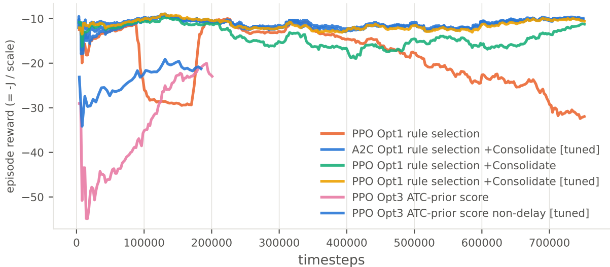
on_rho075: training curves (each line one seed)
