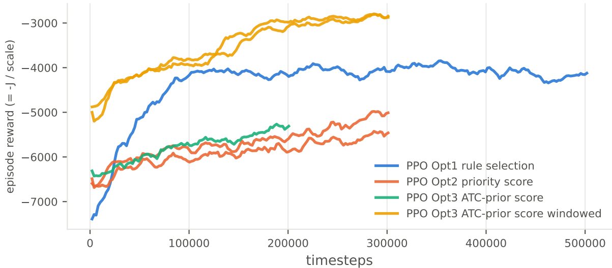
off_tf08: training curves (each line one seed)
