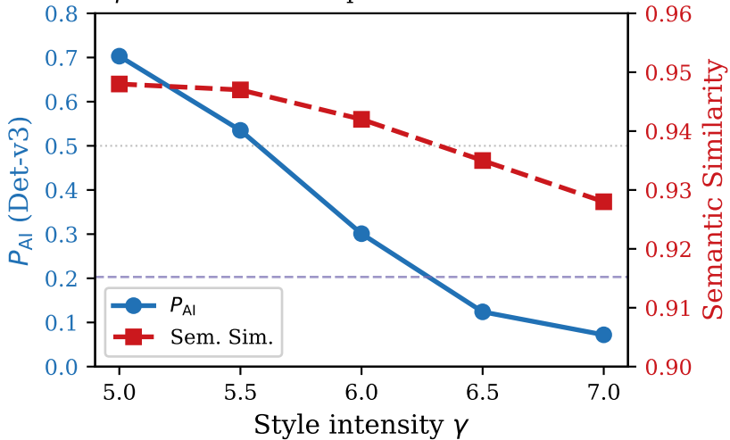
\gamma controls evasion--preservation trade-off
