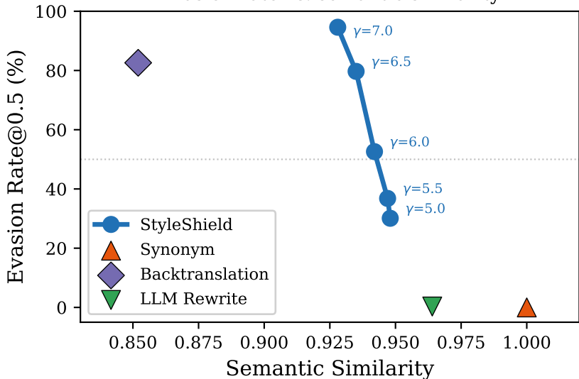
Evasion rate vs. semantic similarity
