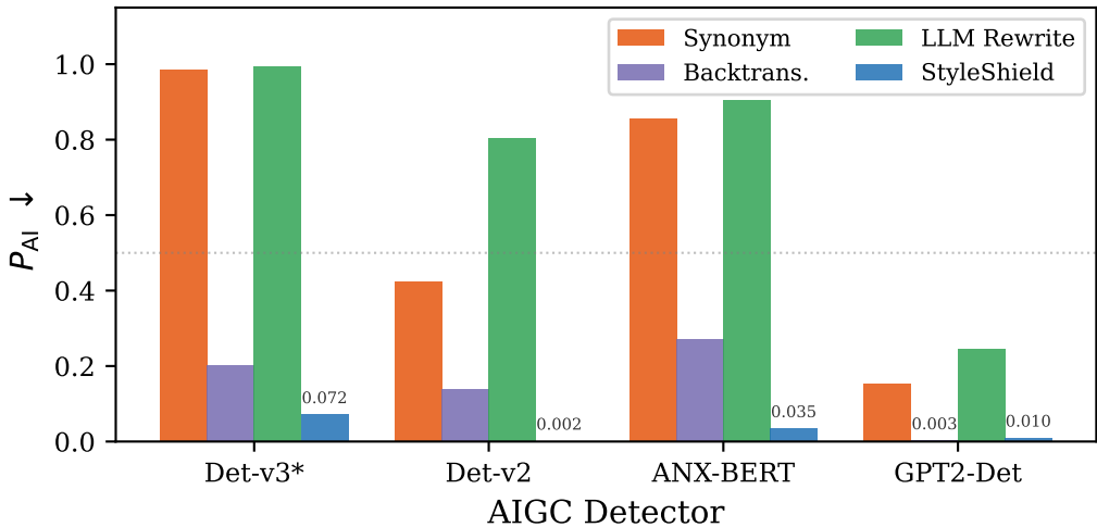
Cross-detector generalization ( \gamma=7.0 )
